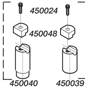
Terminal 450024 - Screw 450039 - Short 450040 - Long 450048 - Top
