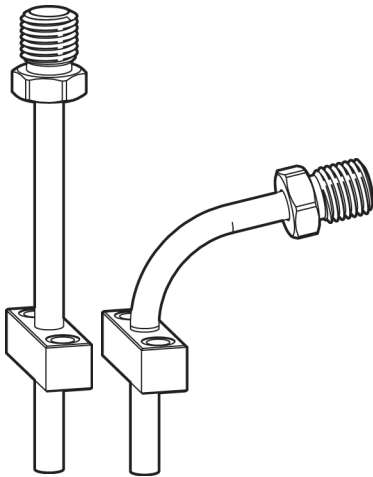
Powder Injectors 5004378-S Straight 5004378-B Bent
